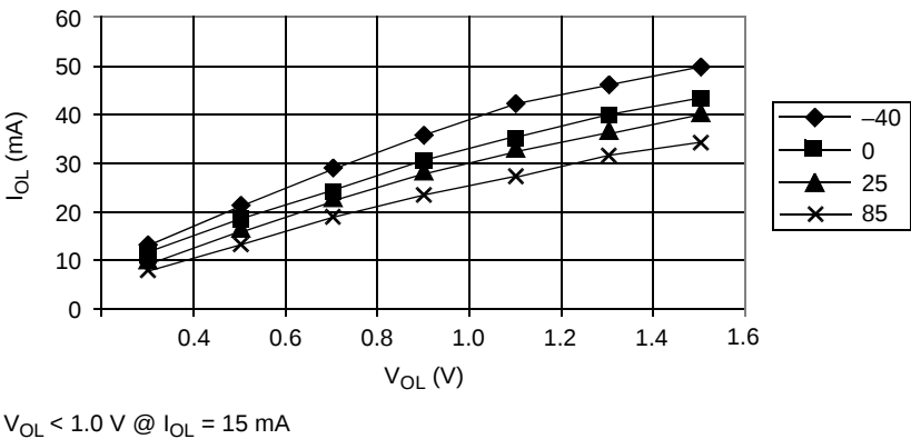
Figure 23-9. Typical Low-Side Driver Characteristics – Port PTC1–PTC0 ( V_{DD} = 4.5\text{ Vdc} )
