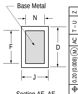
Section AE-AE
