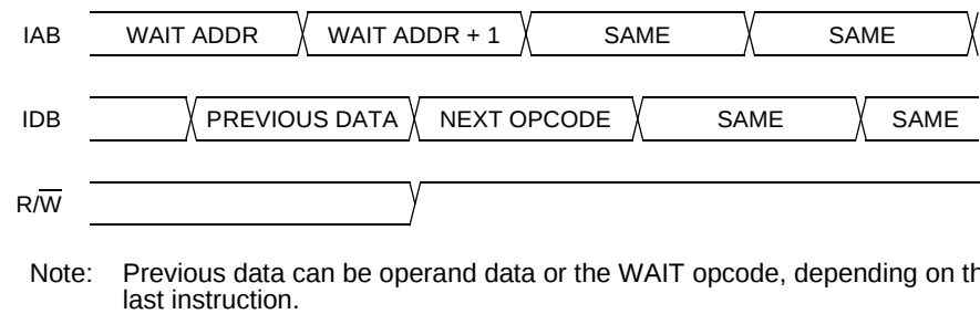
Figure 19-15. Wait Mode Entry Timing
